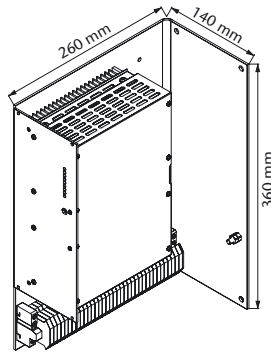
Series SS 15xx Wall mount / approx. 6.3 kg
