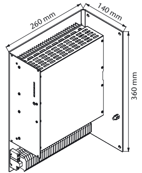
Series SS 35xx Wall mount / approx. 8 kg
