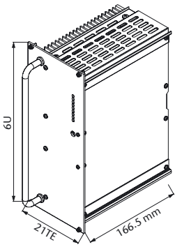
Series SS 15xx Eurocassette / approx. 3.3 kg (pluggable module for 19" sub-rack)
