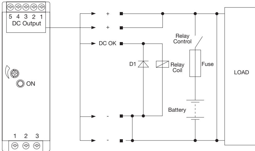
DNR30/60 connection for DC standby system applications
